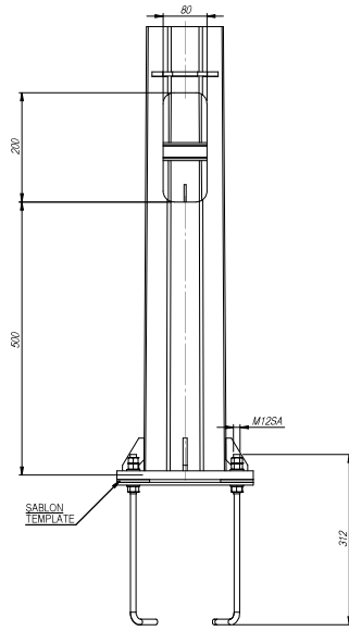
SECTION D-D SCALE_1/15 ALT MONTAJ VE KAPAK DETAY ANCHOR CAGE AND COVER DETAIL
