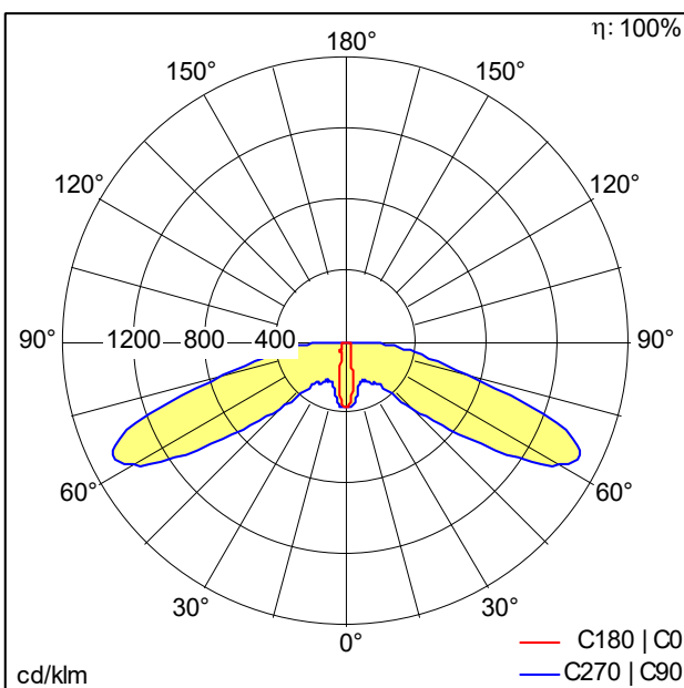
D43511_RESCLITE_PRO_MSC_ESC_HP_E1D_WH_IP65.idt
