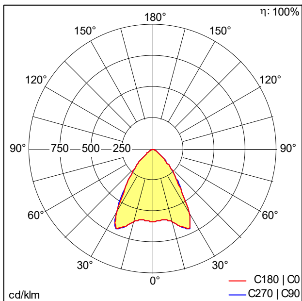
D43023_MIRL_LAY_3800-840_M600Q_NB_EVG_WH.Idt
